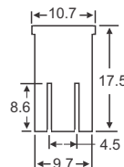
Mc case Slotted Fuse
