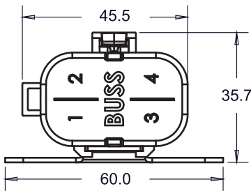
CFH-ALS (Long cover & Side Bracket)
