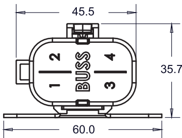
CFH-ASS (Short cover & Side Bracket)
